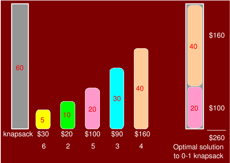
Figure 7.10: Optimal solution for the 0-1 knapsack problem
