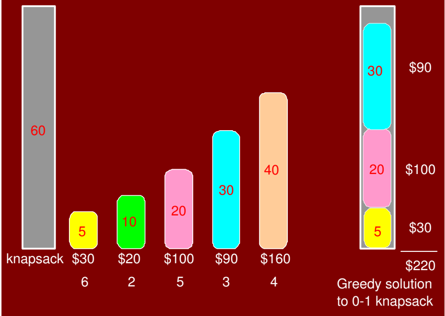
Figure 7.9: Greedy solution for the 0-1 knapsack problem (non-optimal)
