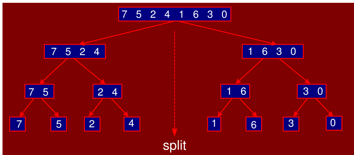
Figure 3.1: Merge sort divide phase
